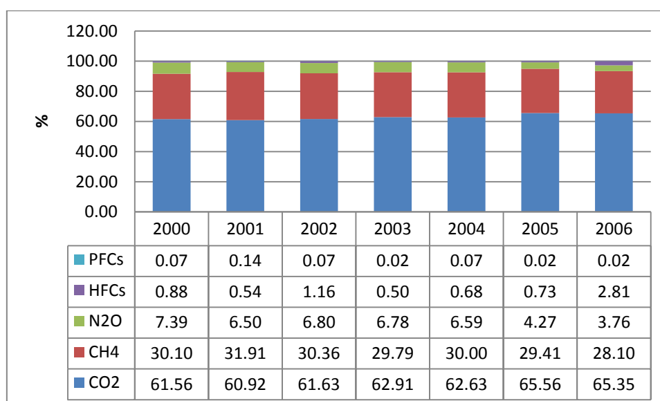
Figure 2.2 - Share by gas of GHG emissions
