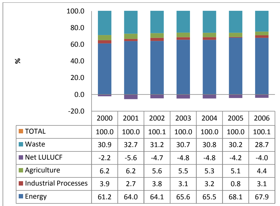
Figure 2.3 - Share of GHG emissions by sector
