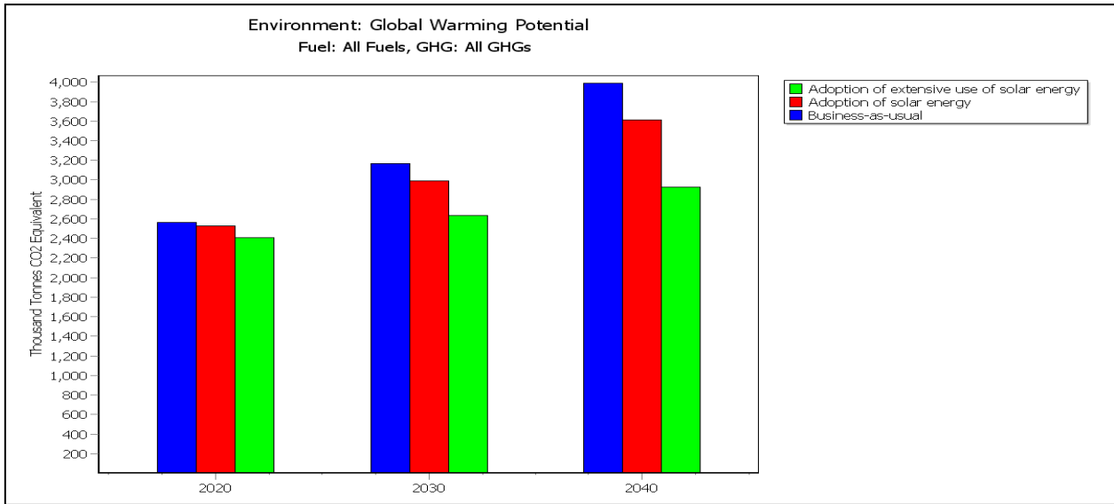
Figure 4.10 - Emissions (Gg CO 2 -eq) by fuel from Electricity generation category under alternative share of solar energy as estimated by the LEAP Model
