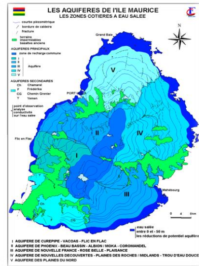
Figure ES 3 - Aquifers of Mauritius (Courtesy : WRU)
