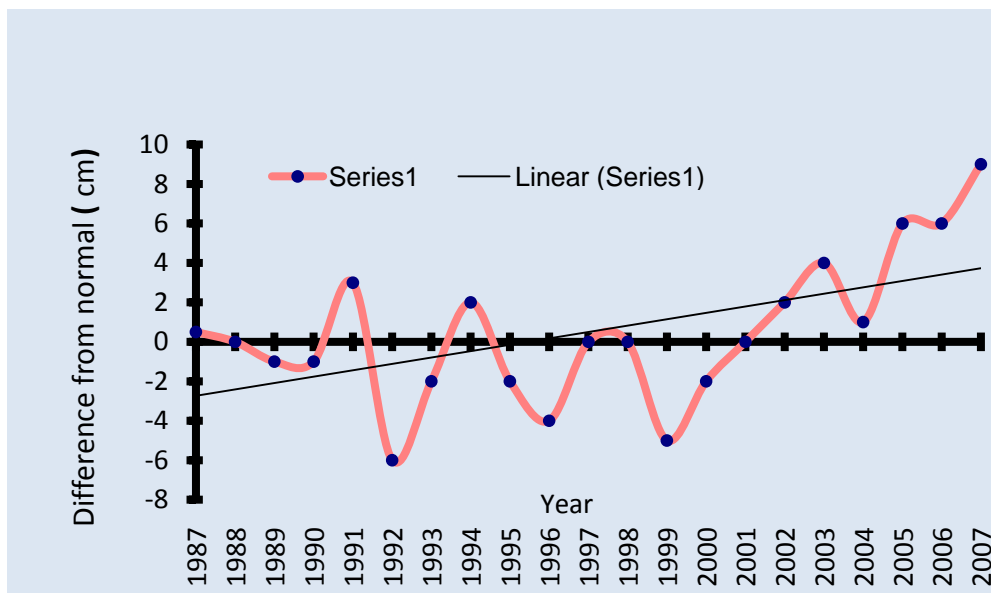
Figure 5.4 - Sea level rise monitored at Port Louis
