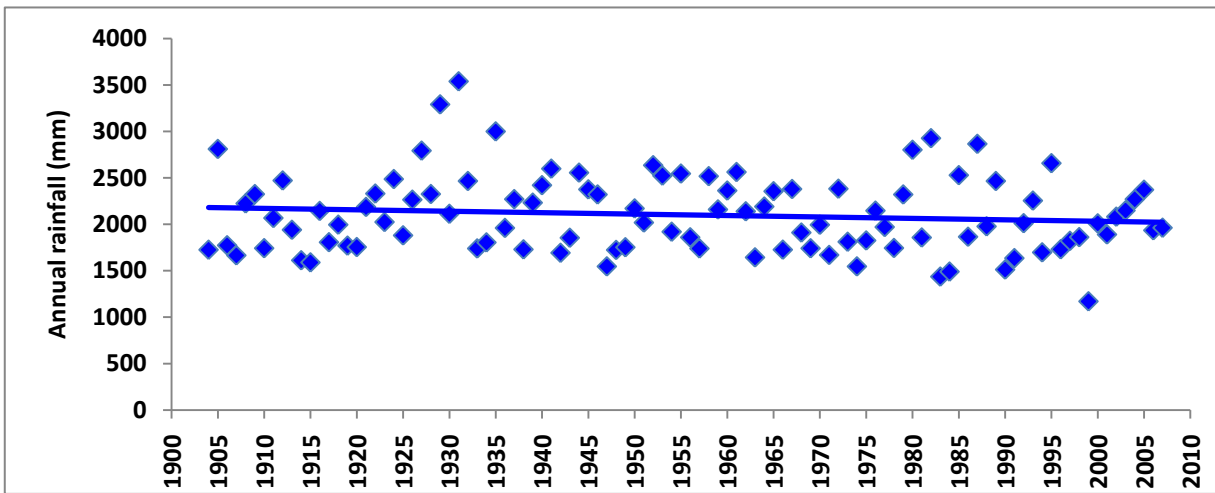
Figure 1.4 - Long-term annual rainfall over Mauritius
