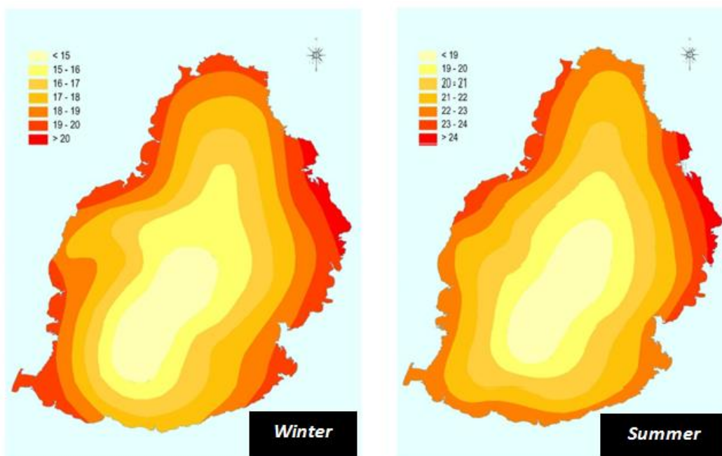
Figure 1.3 - Distribution of mean minimum temperature (°C) over Mauritius
