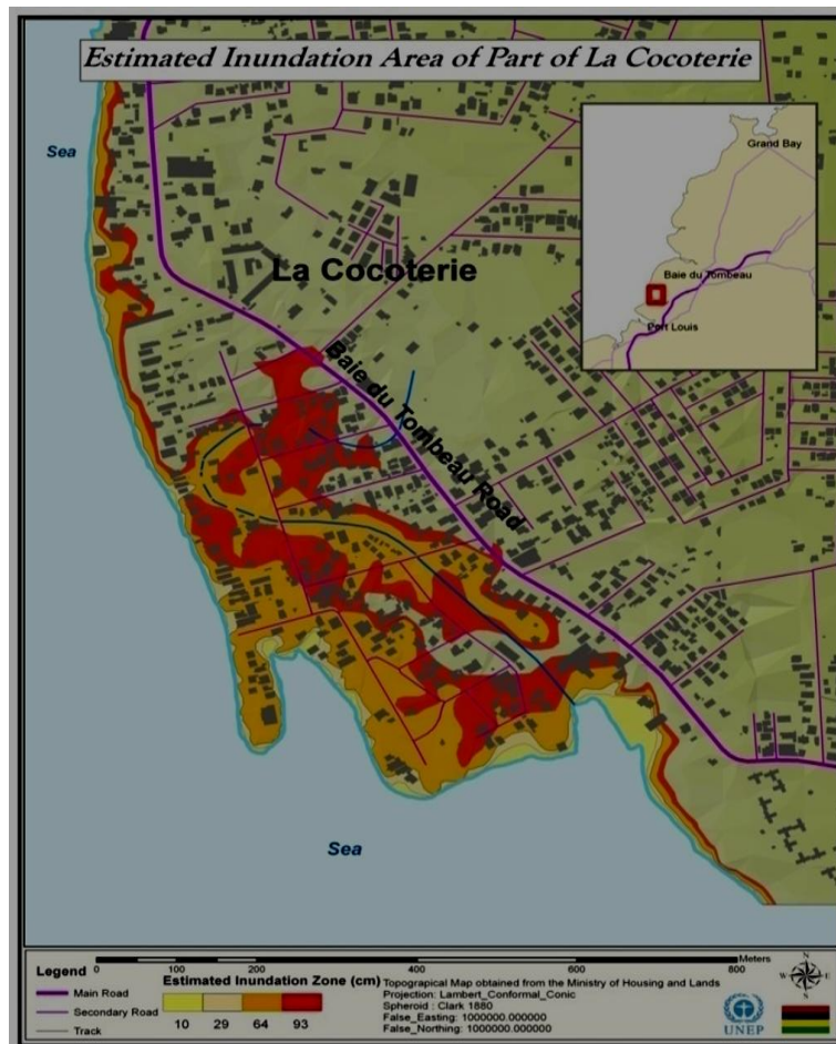
Figure 5.6 - Inundation map generated for the Baie du Tombeau area in the event of 4 m wave run up
