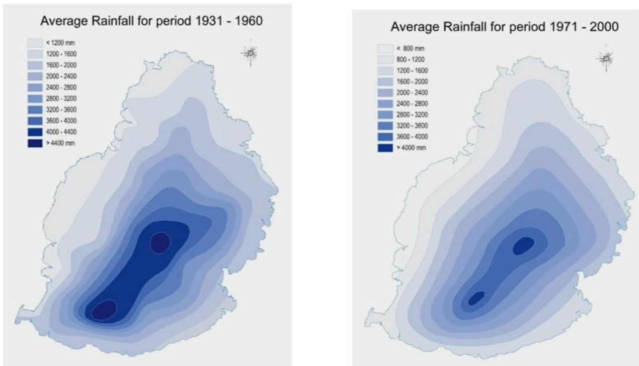
Figure 1.5 - Rainfall distribution over Mauritius for periods 1931-1960 and 1971-2000
