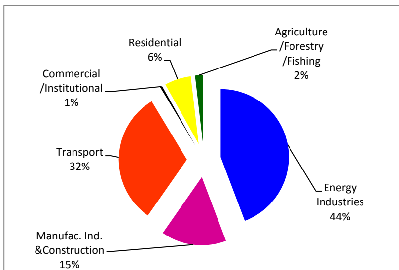
Figure 2.5 - Share of emissions of the Energy sub-sectors (2000)
