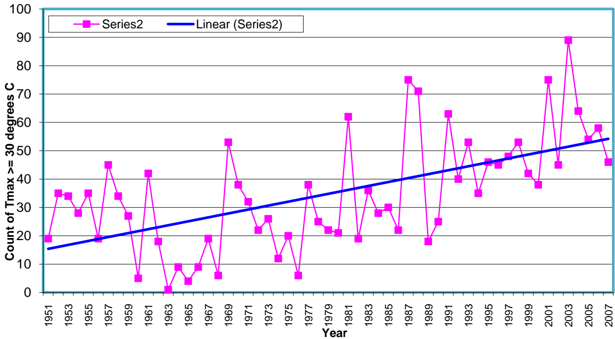
Figure 5.2 - Annual count with Tmax >= 30 °C at Plaisance (Source: Mauritius Meteorological Services)
