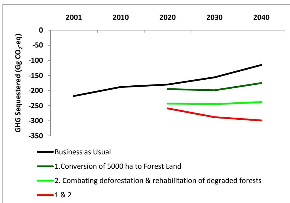
Figure 4.5 - Projected GHG sequestration with mitigation options in the LULUCF sector (The numbers in the legend refer to the Options in Table 4.9)
